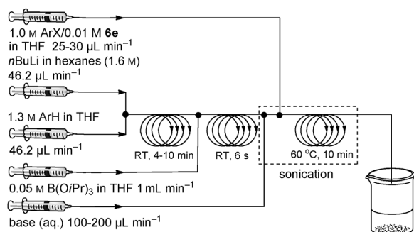
Figure 4. Continuous-flow setup for the lithiation/borylation/Suzuki–Miyaura cross-coupling sequence of heteroarenes with aryl halides.
